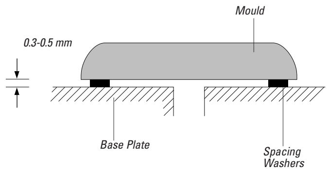
Fig. 1.15b: Slot Design Recommendations
