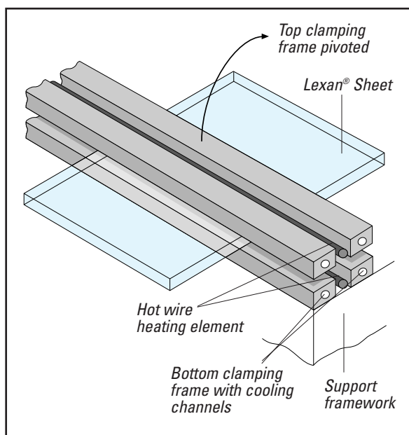
Fig.1.18: Typical Set-up for Hot Line Bending
