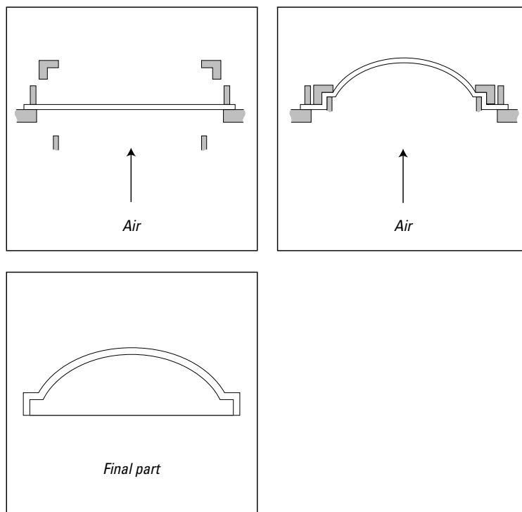
Fig. 1.16: Free-blown Domes
