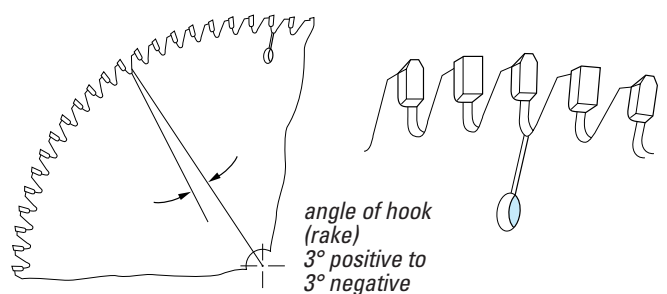
Fig. 2.2: Typical Tungsten Carbide Tipped Circular Saw suitable for Lexan® sheet products
